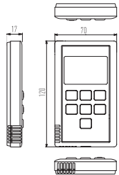
SIMPLIFIED REMOTE CONTROLLER (CZ-RE2C2)
