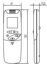
SEPARATE RECEIVER FOR WIRELESS REMOTE CONTROLLER (CZ-RWSC3)
