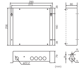
COMMUNICATION ADAPTOR (CZ-CFUNC2)
