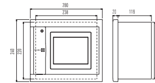
INTELLIGENT CONTROLLER (CZ-256ESMC2)
