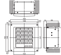
LONWORKS INTERFACE (CZ-CLNC2)
