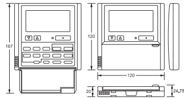
TIMER REMOTE CONTROLLER (CZ-RTC4)
