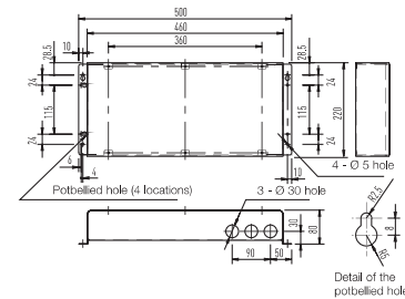
LONWORKS INTERFACE (CZ-CLNC2)
