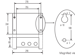
SERI-PARA I/O UNIT FOR OUTDOOR UNIT (CZ-CAPDC2)
