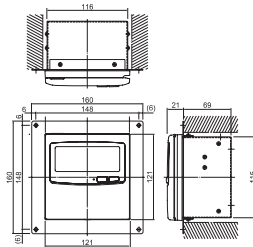
SYSTEM CONTROLLER (CZ-64ESMC2)
